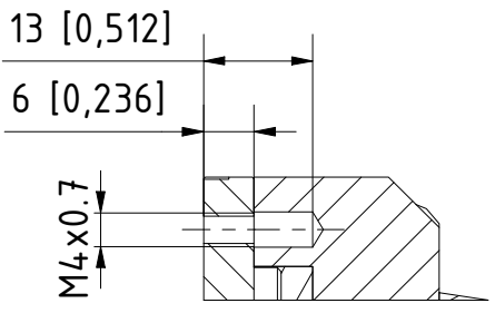
A-A View for bolt hole
